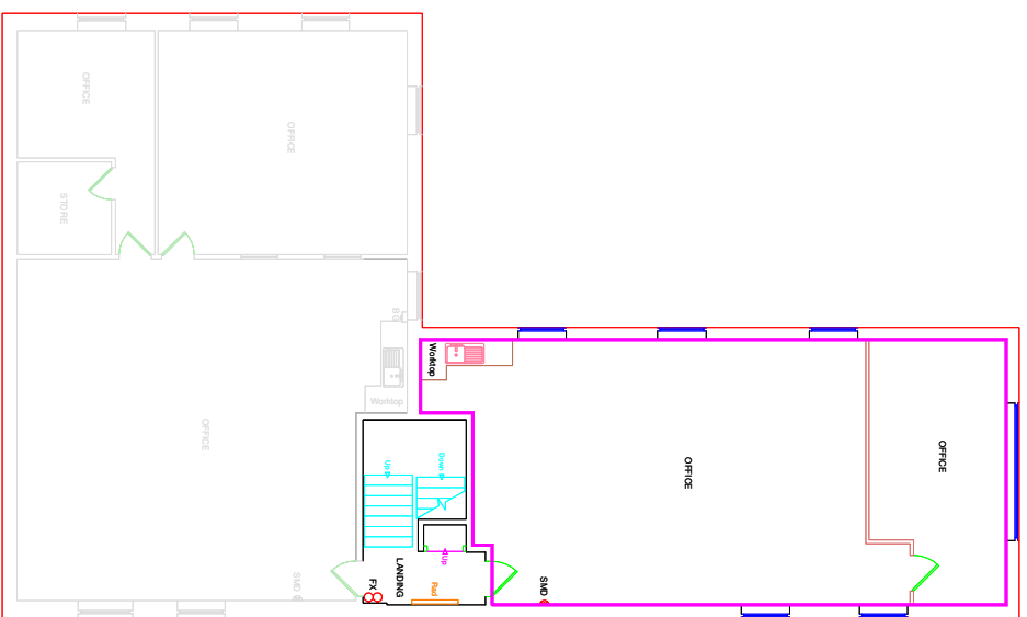
BLOCK F THE CORN HOUSE FIRST FLOOR
